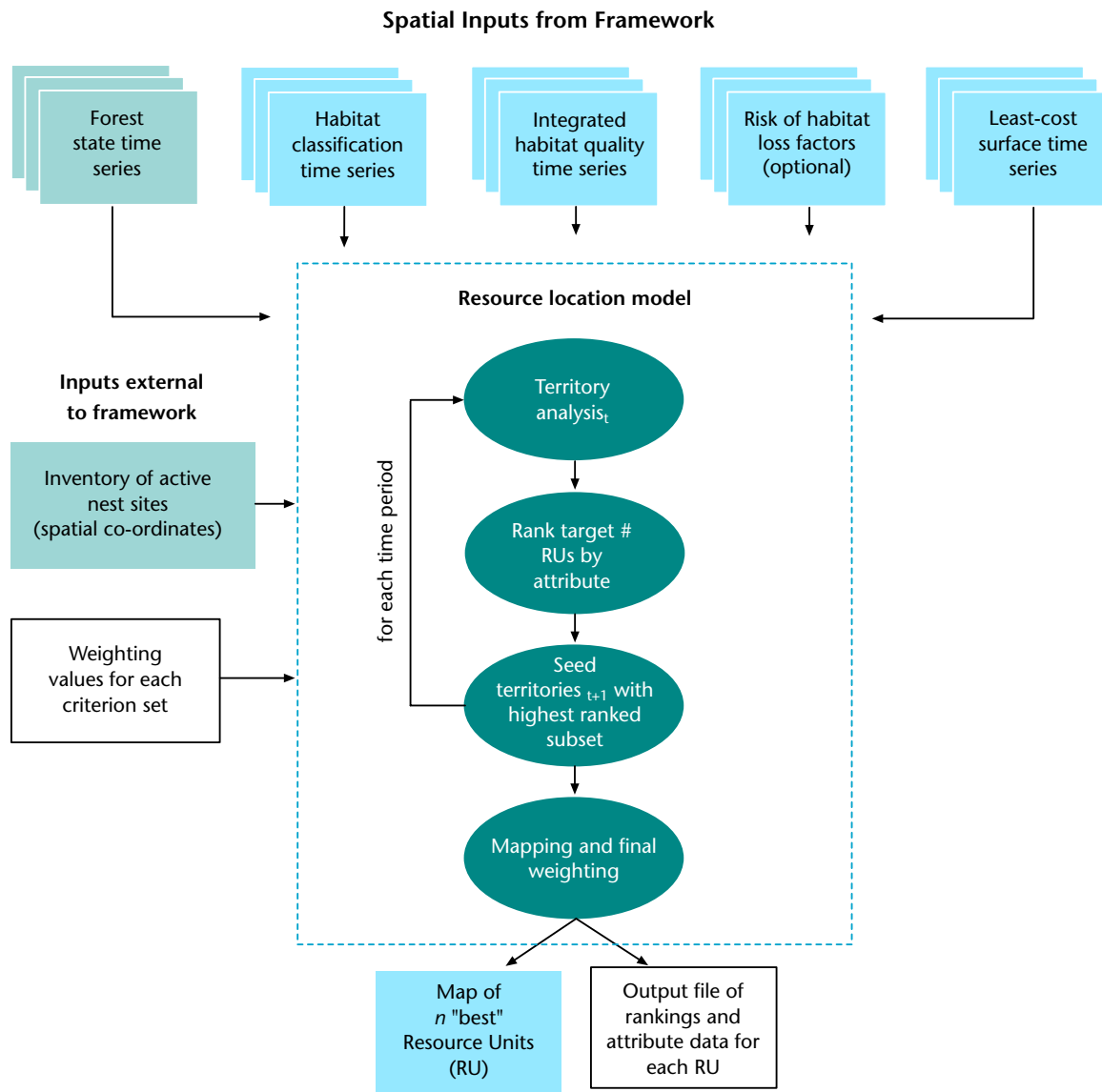
FIGURE 25 Conceptual diagram of the RLM's components, main inputs and outputs, and logic flow.
