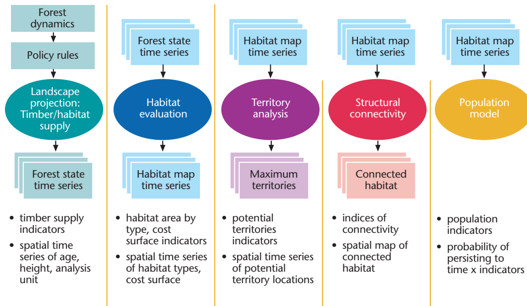
FIGURE 3 Implementation of the modelling components of the analysis framework as a "pipeline." Interpretation of graphics as in Figure 2. List bullets indicate indicators stored as stratified text files. All components operate at a spatial extent of a geographic range, and a grain size defined by the finest resolution in the data (see text).
