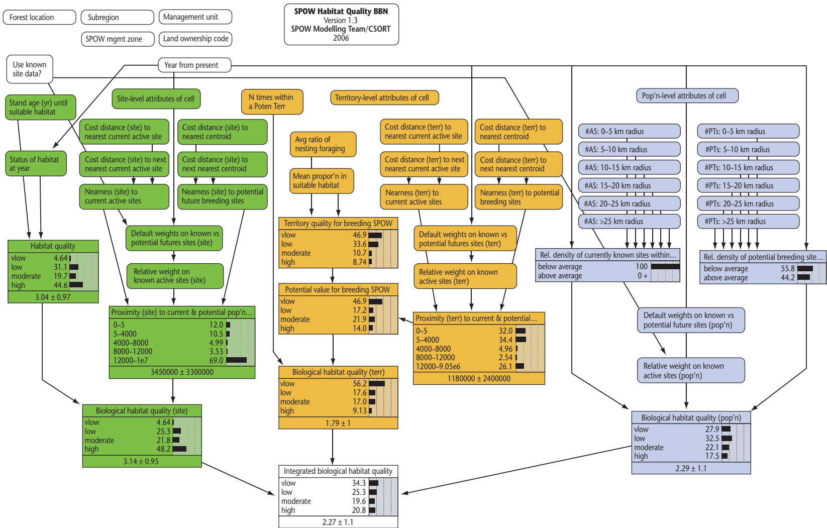
FIGURE 22 The full habitat quality BBN as implemented in the framework for the Spotted Owl case study. All nodes are shown here with their scale-contexts identified using the colour scheme presented in Figure 21. Nodes representing attributes calculated from analysis of landbase data or derived from other components of the framework are shown as simple boxes with labels. Nodes containing rules are shown as boxes containing weightings (black bars) or degrees of belief in each state. The overall expected value (value weighted by the numerical probability of each state ± SD) is shown at the bottom of each node. Poten Terr = potential territories.
