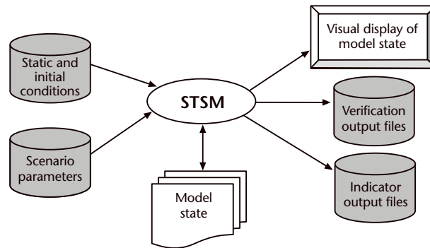
FIGURE 5 Conceptual structure of the spatially explicit timber supply model. The central circle represents the main STSM model components. Grey cylinders represent input/output text files. Stacked icons represent time series of inputs/outputs, generally stored as maps or sometimes as text files. The 3-D box indicates the user interface of SELES.
